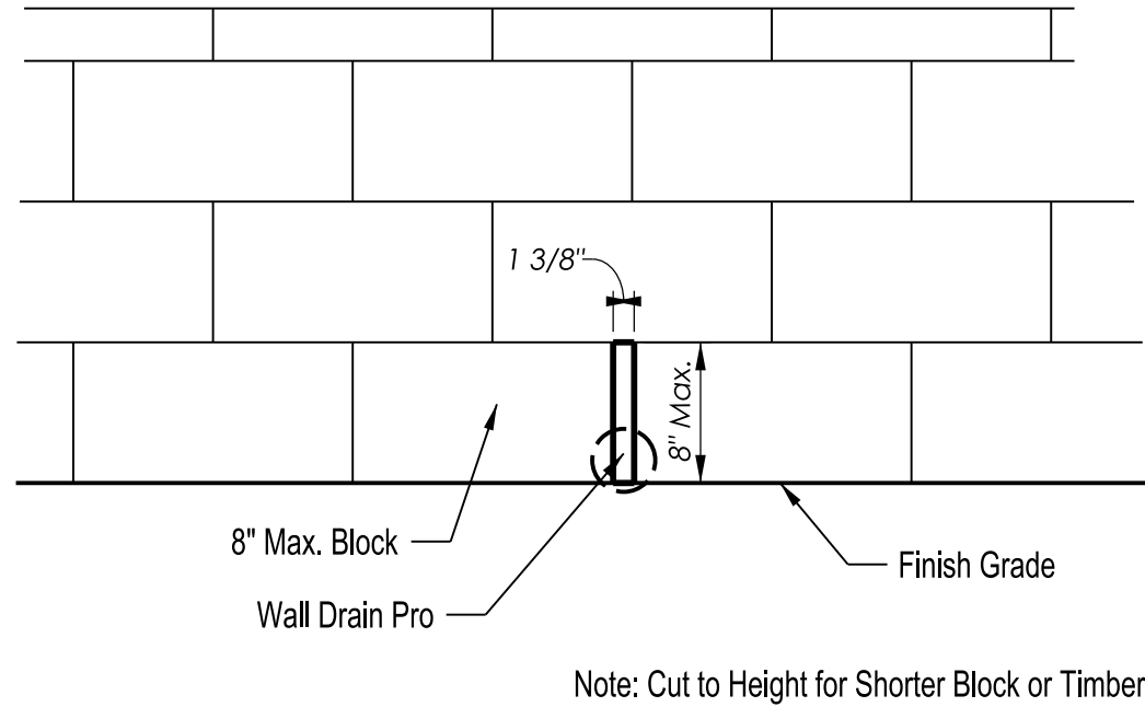
Wall Elevation
