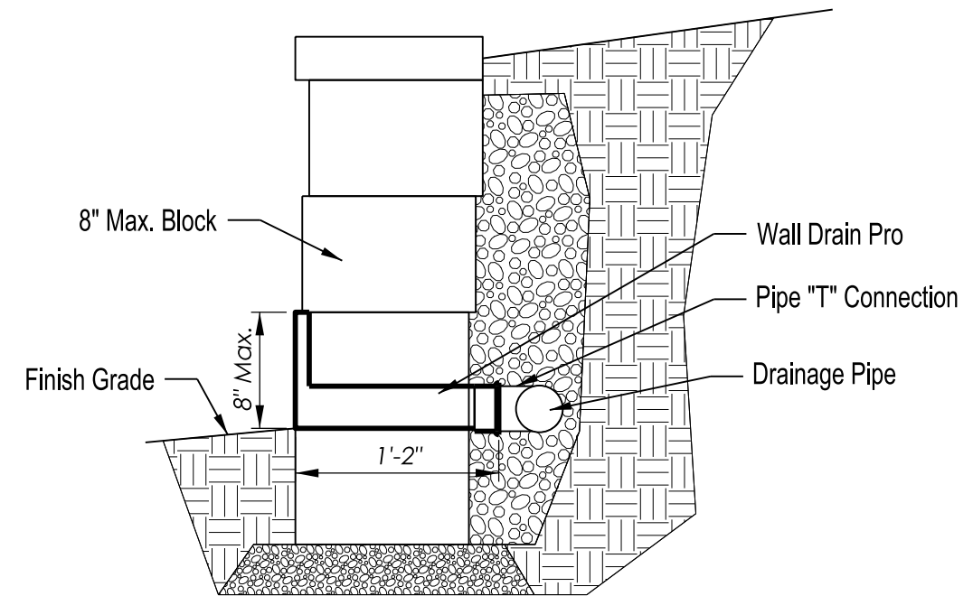
Wall Section
