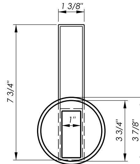
Wall Drain Pro Detail - End View
