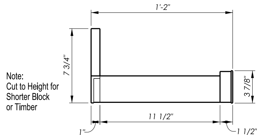
Wall Drain Pro Detail - Side View
