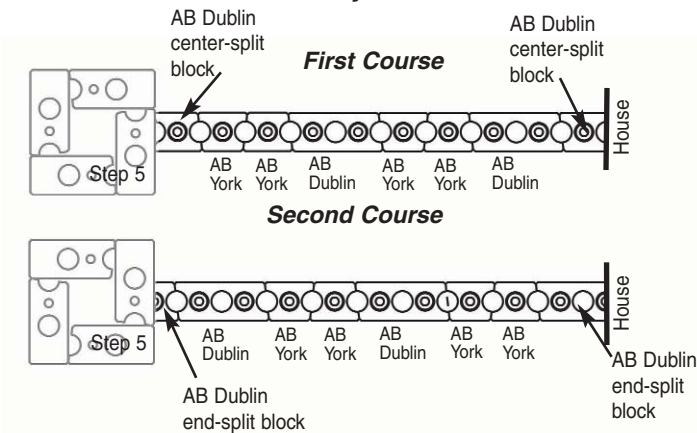
Figure 6: 2nd Wall Panel Course Layout
